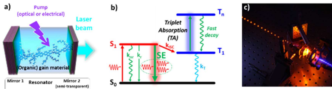
Figure 1: a) General structure of a laser. b) Simplified Jablonski diagram with dominant mechanisms under optical pumping: SE = stimulated emission, k_r/k_{nr} = radiative/nonradiative decay rates of singlet state, k_T = triplet state decay rate, k_{isc} = intersystem crossing rate. c) Image of optically-pumped organic Laser beam (LPL).
